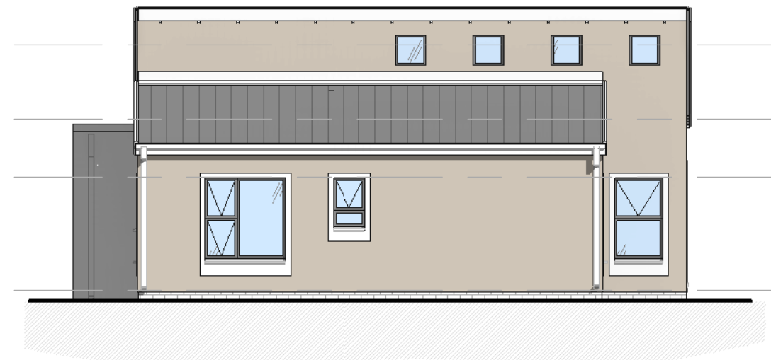
TYPICAL UNIT TYPE A - BACK ELEVATION
