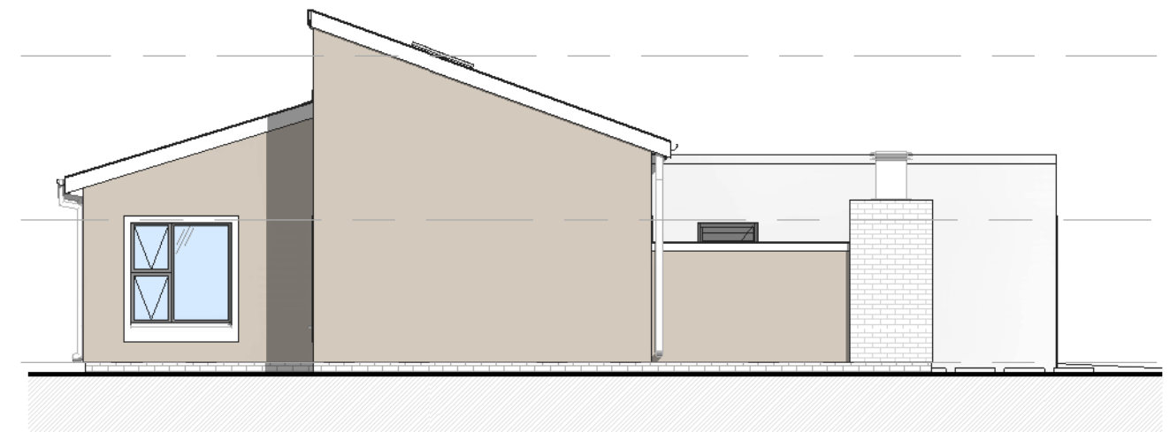
TYPICAL UNIT TYPE A - SIDE ELEVATION
