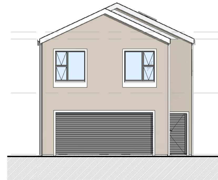
TYPICAL UNIT TYPE C - FRONT ELEVATION
