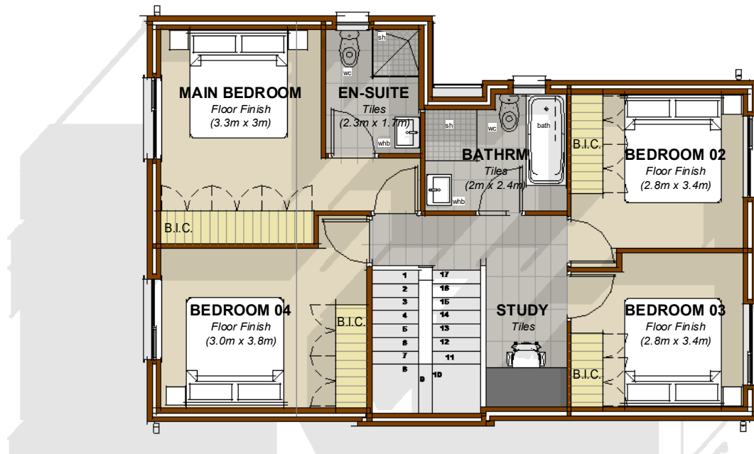
TYPICAL UNIT TYPE C - FIRST FLOOR PLAN
