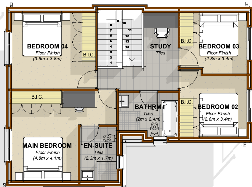
TYPICAL UNIT TYPE D - FIRST FLOOR PLAN
