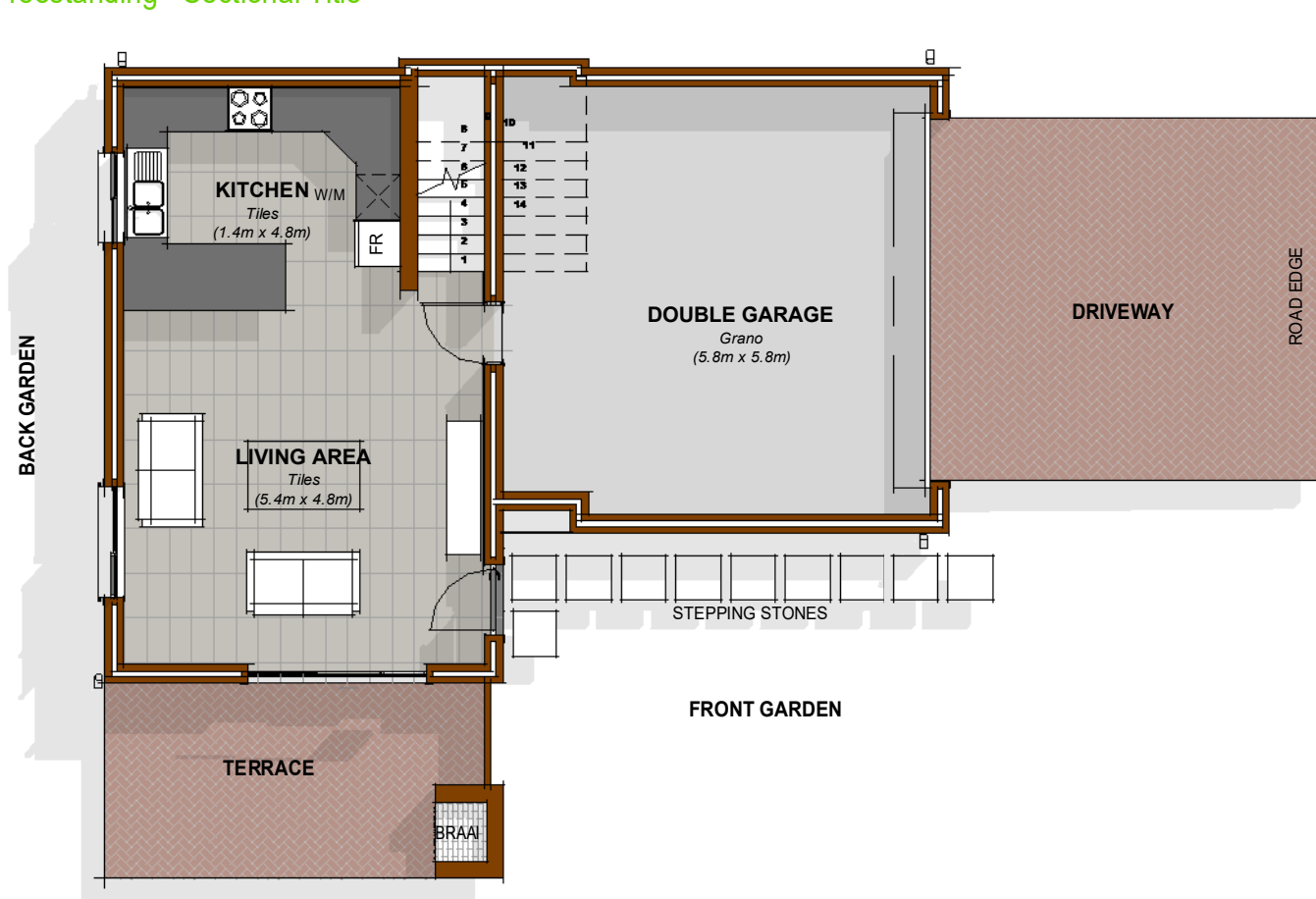
TYPICAL UNIT TYPE D - GROUND FLOOR PLAN
